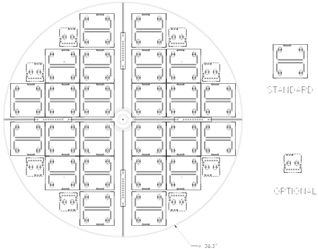
XLC 1520HE RACK LAYOUT
