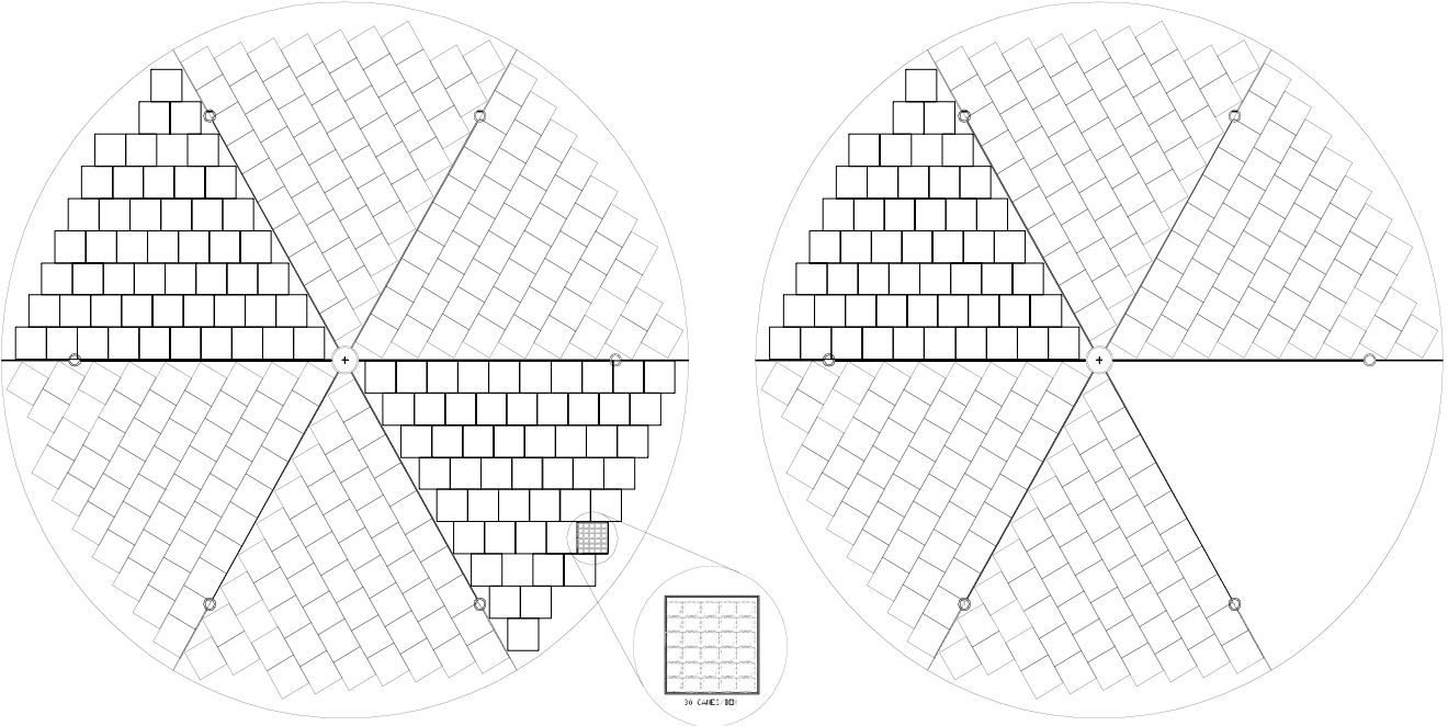
XLC 1830 2T SUC-1 LAYOUT
