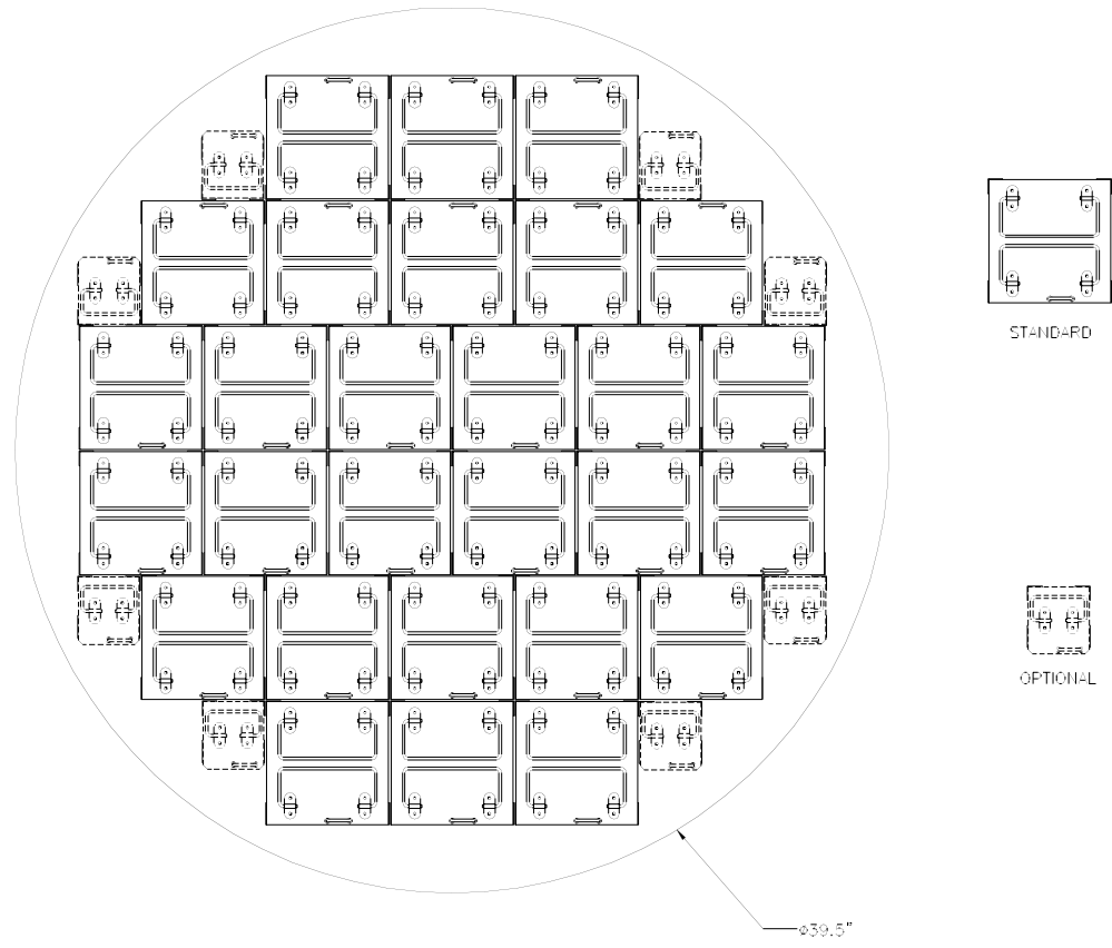
XLC 1841 RACK LAYOUT
