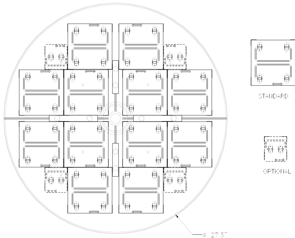
XLC 810HE RACK LAYOUT
